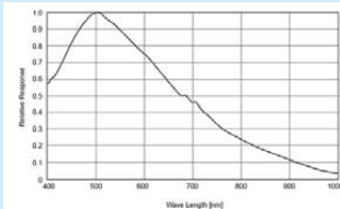
Spectral Sensitivity for G0531B
